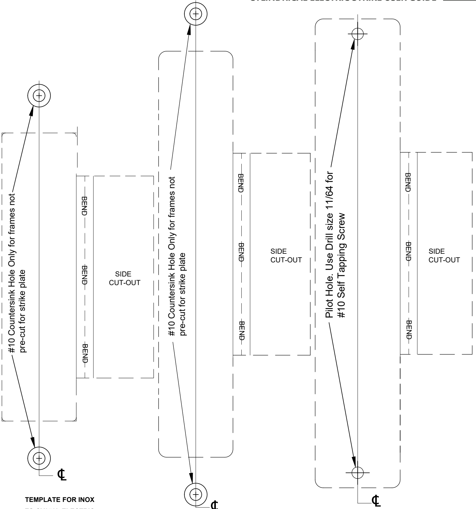
TEMPLATE FOR INOX ES-CY079L ELECTRIC STRIKE
